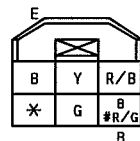
0912-102 REAR WINDOW DEFROSTER SWITCH (F)
