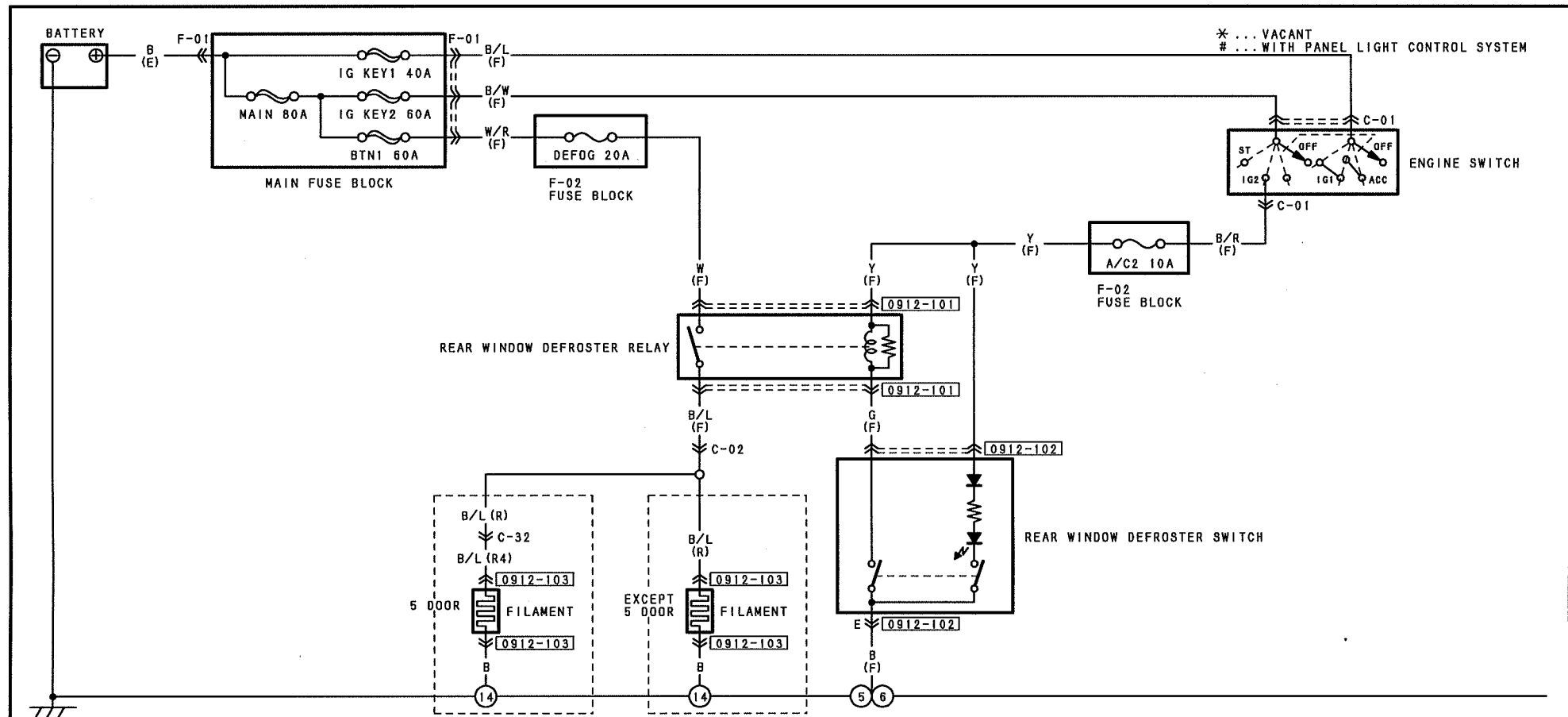
0912-101 REAR WINDOW DEFROSTER RELAY (F)
